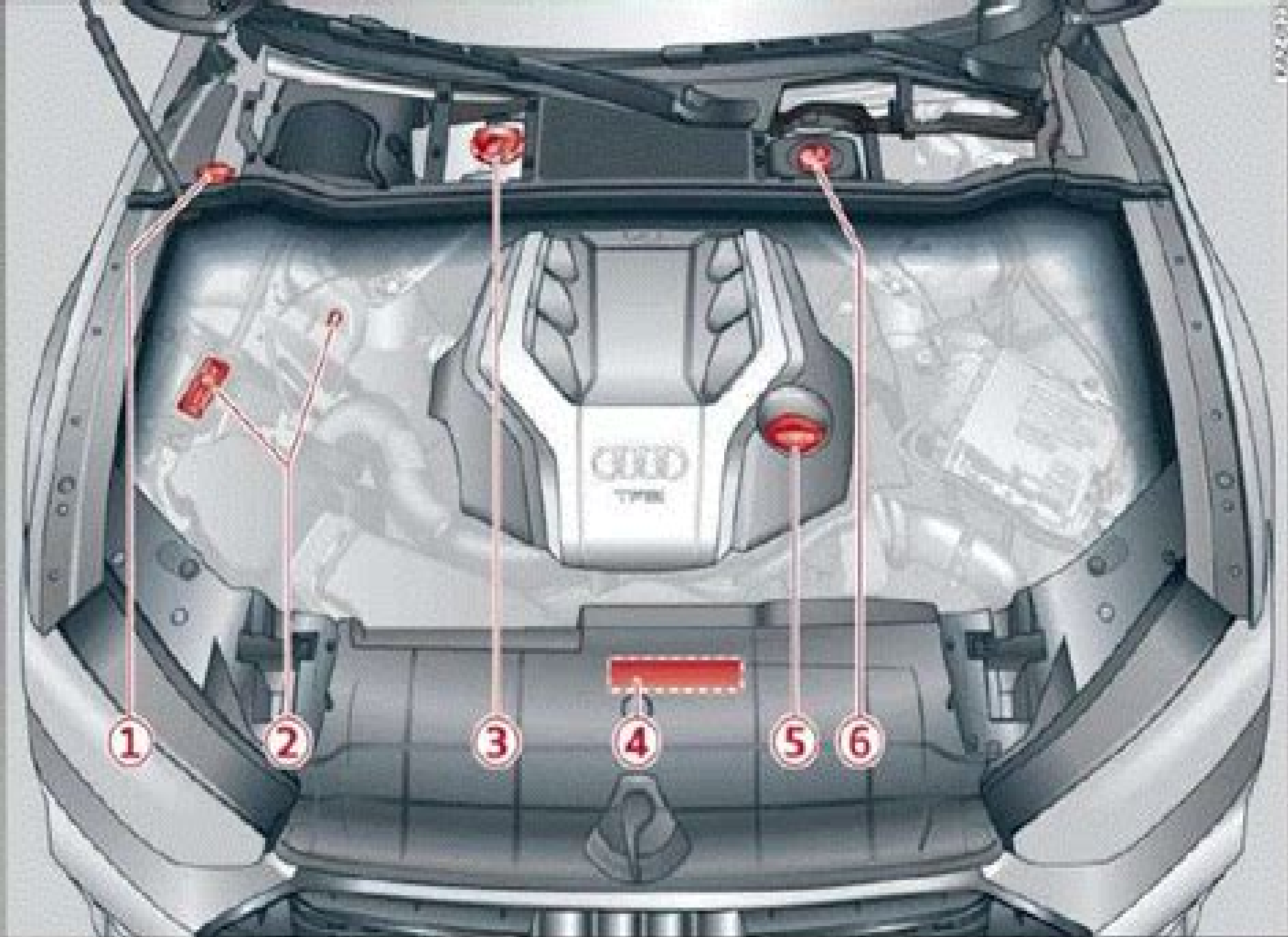
Fig. 164 Engine compartment overview: diagram
