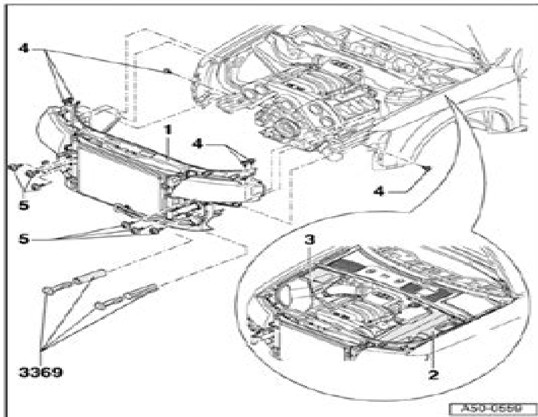
Fig. 1: Lock Carrier Overview
