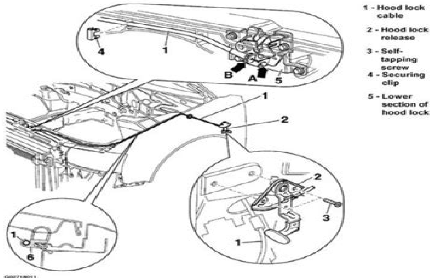
Fig. 10: Removing And Installing Hood Lock Cable
