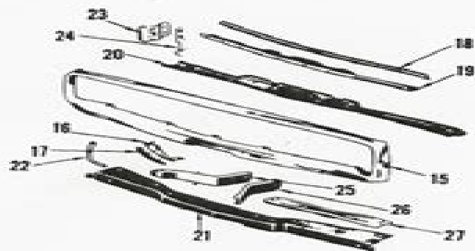
FIG. D — FRONT BUMPER — CHARGER
