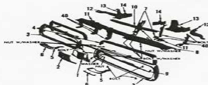
FIG. C — FRONT BUMPER — EXC. CHARGER
