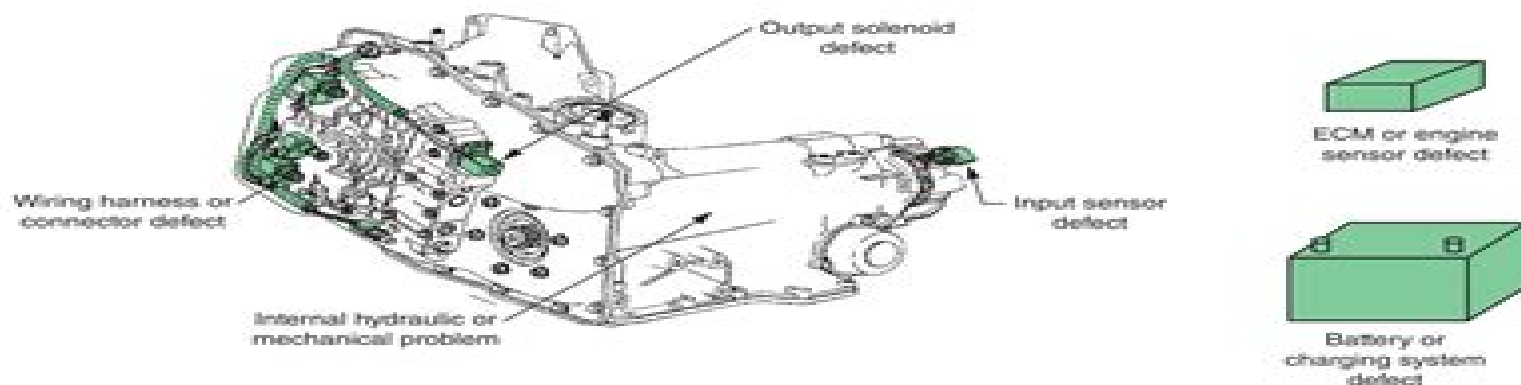
Figure 14-1. Possible trouble spots on an electronically controlled transaxle. Remember that conventional problems, such as worn clutches or internal leaks, are just as likely as electronic component failure. (General Motors)
