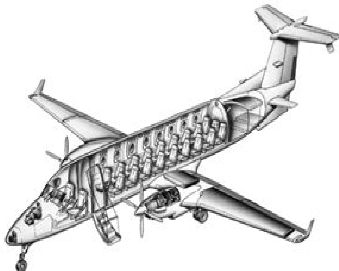
Figure 1-1 1900 Airliner General Arrangement—Series UE
