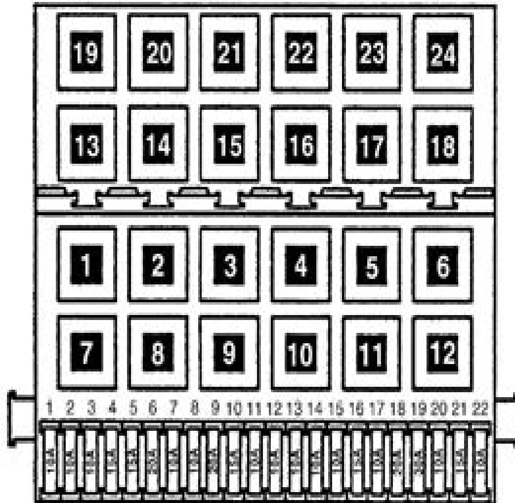
Fuse/Relay Panel
