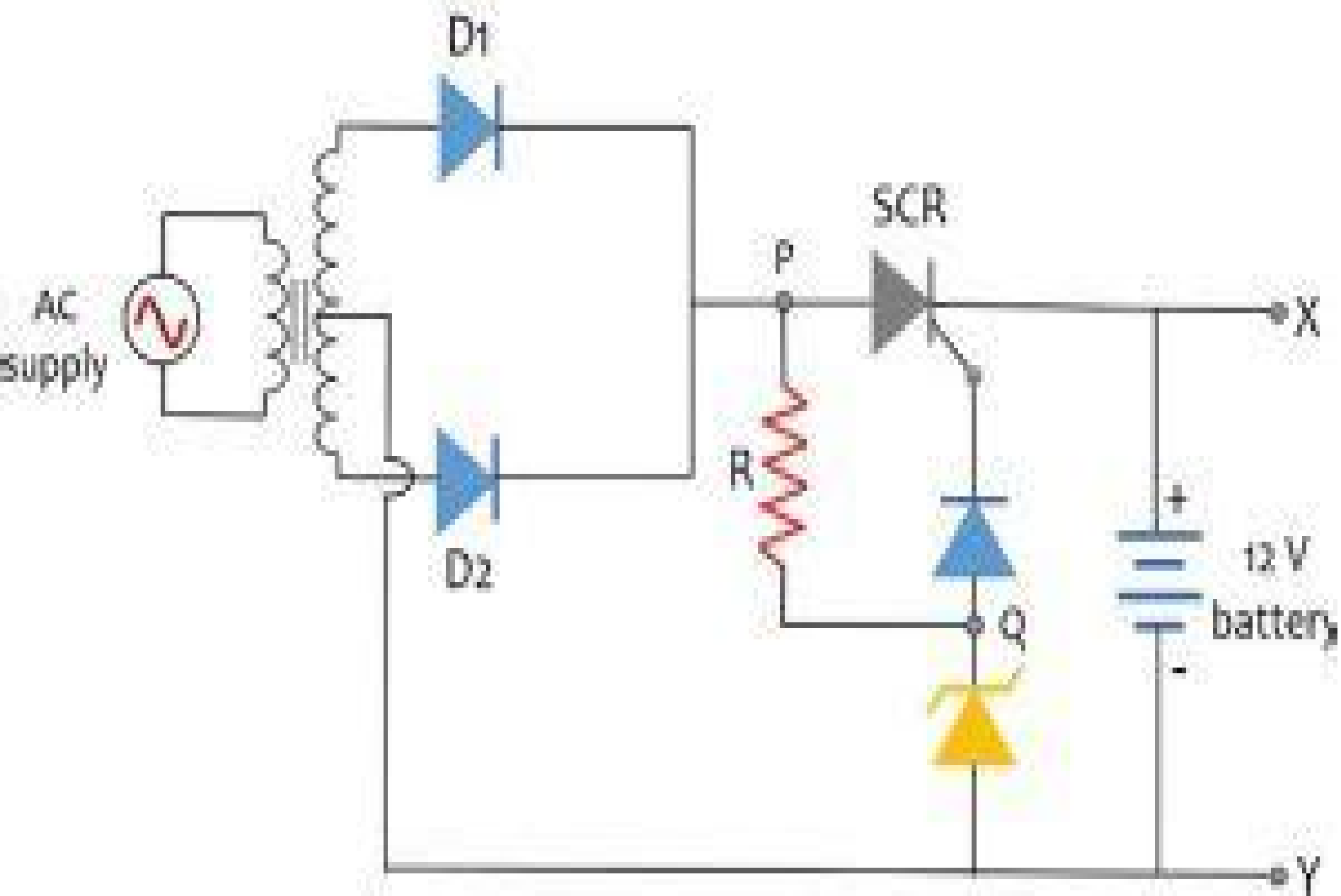
Battery Charger Circuit using SCR
