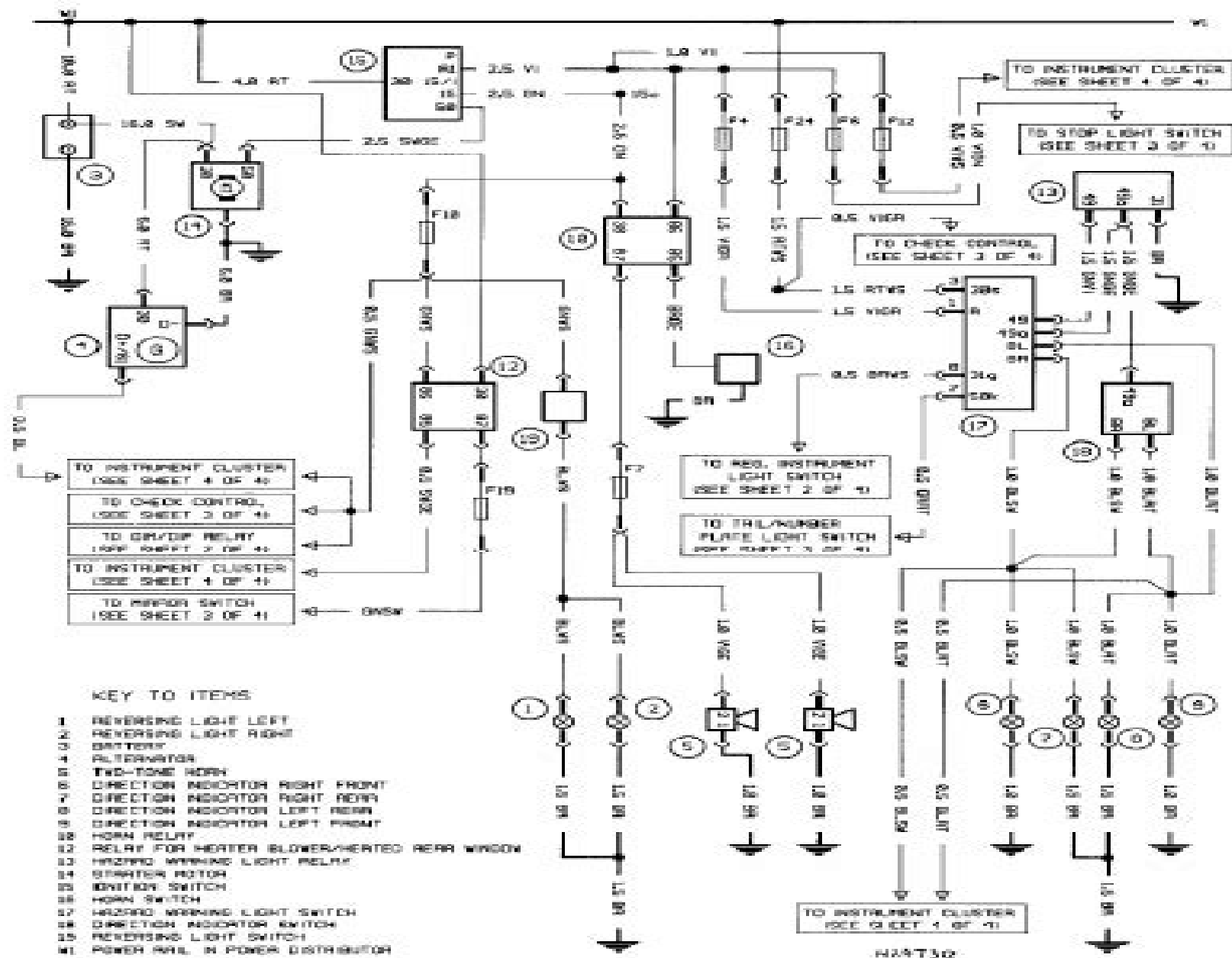
Typical starting, charging, horn, hazard flasher and direction indicators (1 of 4)
