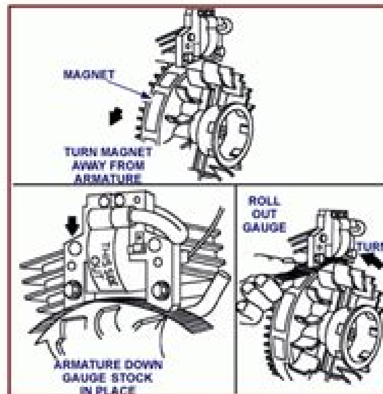
Fig. 13 Adjust Armature Air Gap
