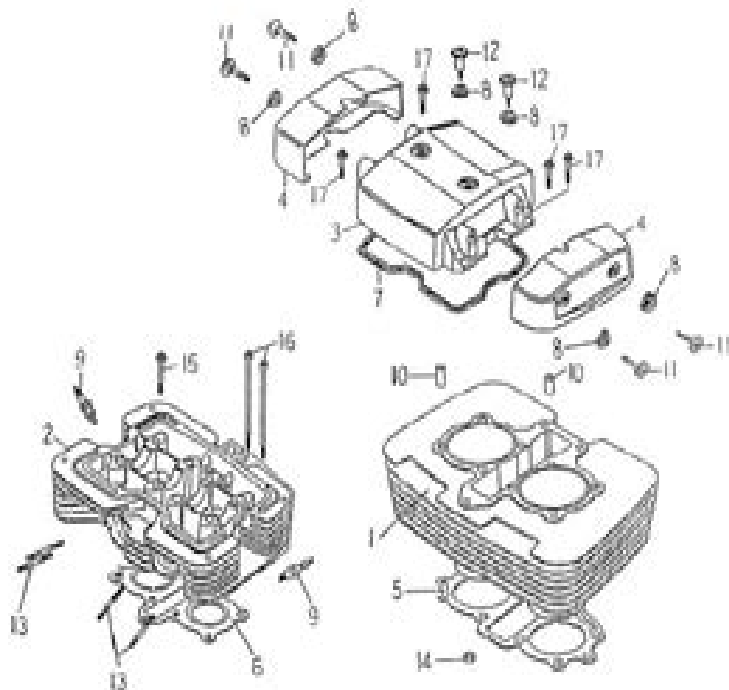
FIG.01 CYLINDER.CYLINDER HEAD
